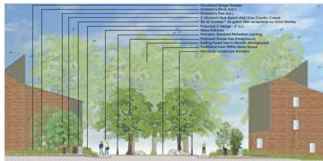
Section B — Section Through Mews
