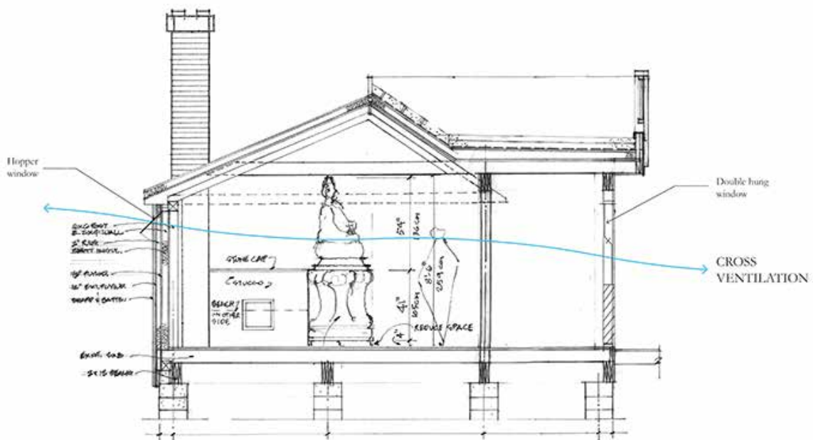
SECTION AT RENOVATED STRUCTURE
