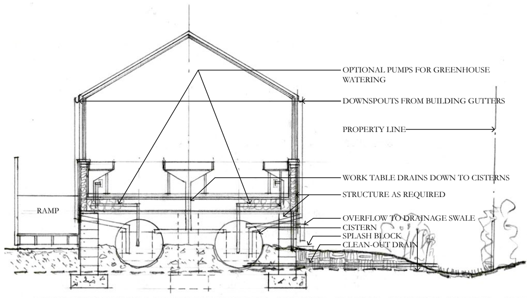
SECTION AT THE GREENHOUSE
