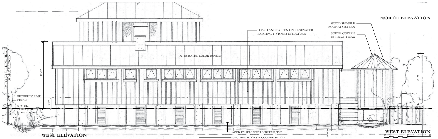
WEST ELEVATION
