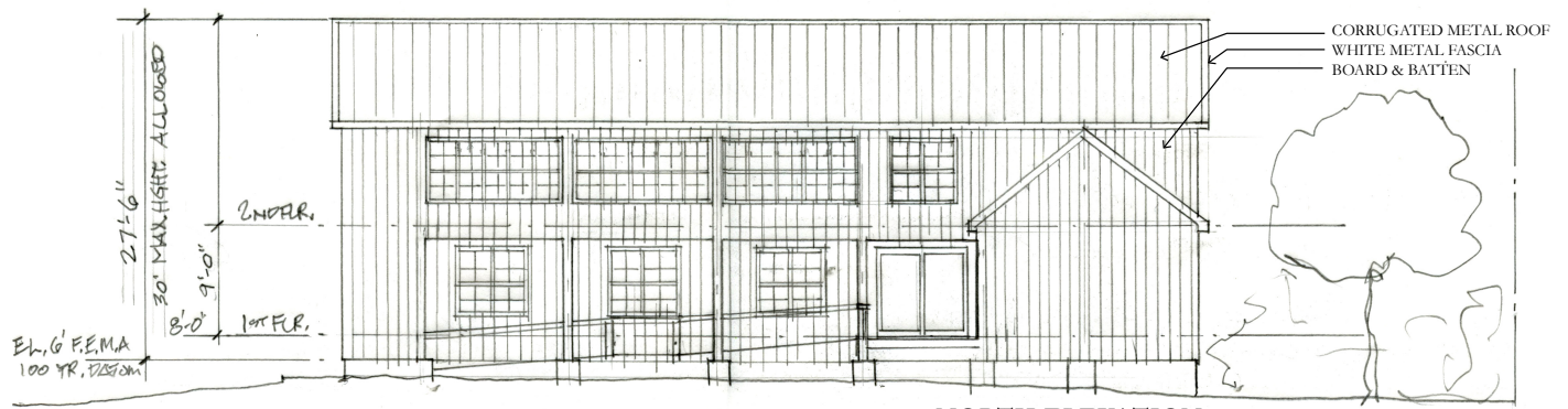
NORTH ELEVATION
