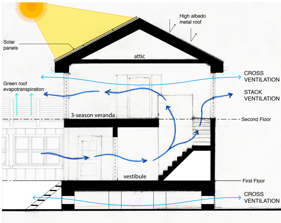
Ventilation & Solar Section Diagram, integrated solar panel and green roof installations
