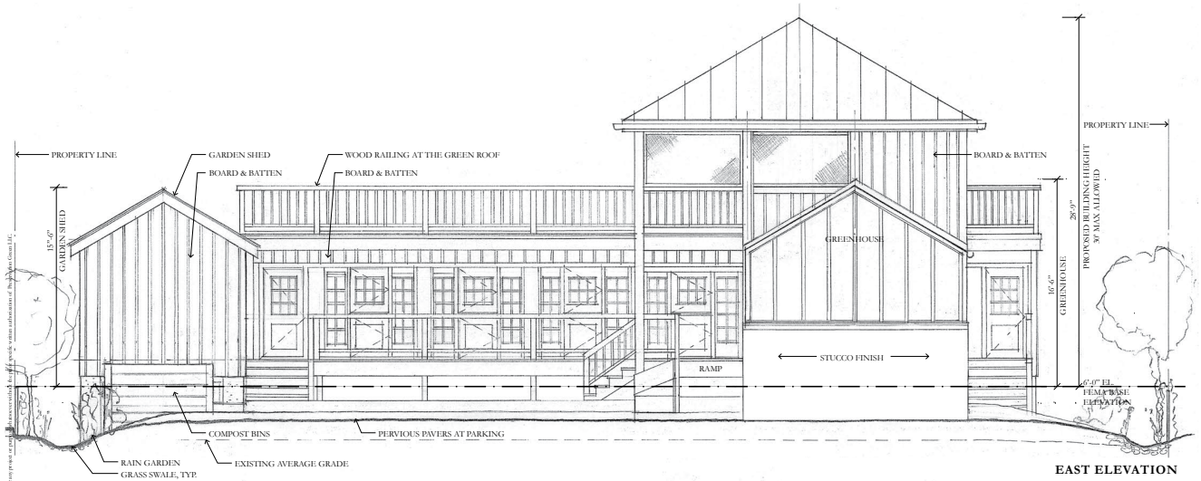
EAST ELEVATION
